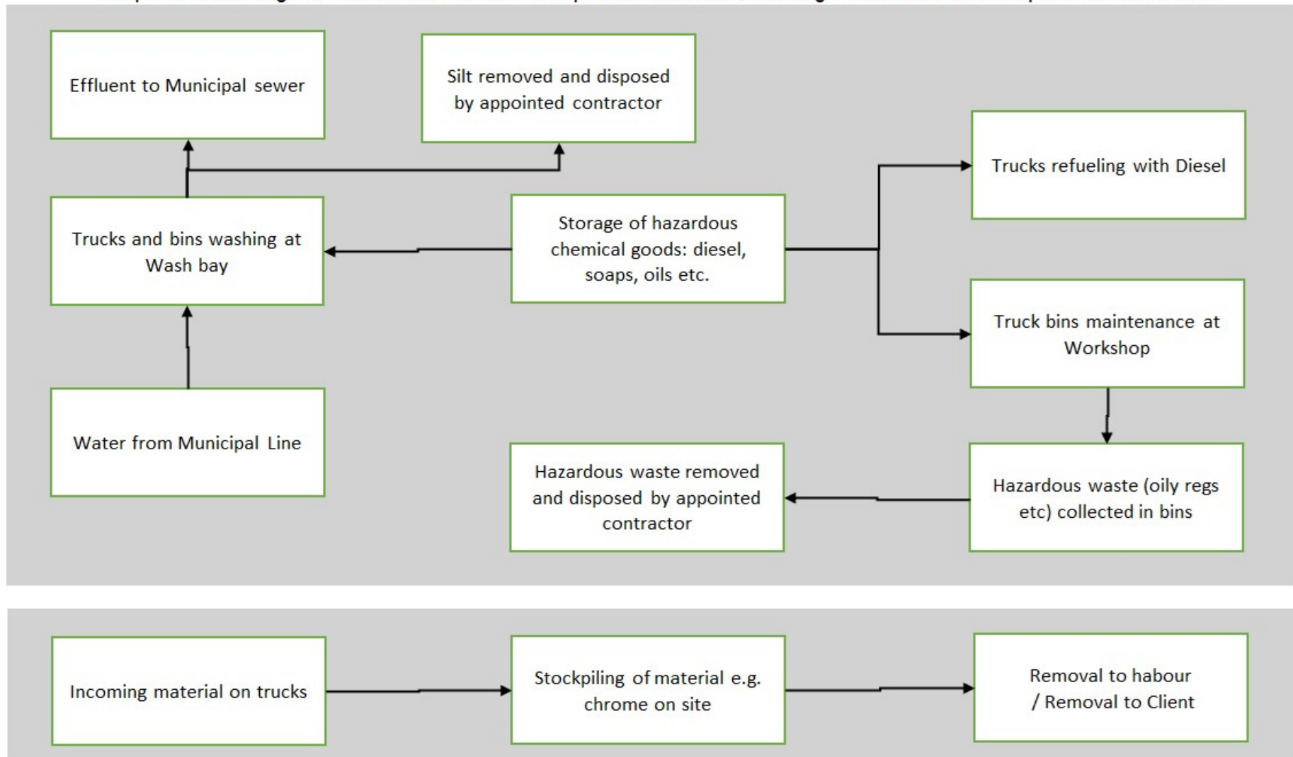
Simplified block diagram with the name of each unit process in a block; showing links between all unit processes or blocks
